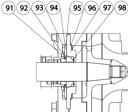
Figuur 3 Mechanical seal S2.
