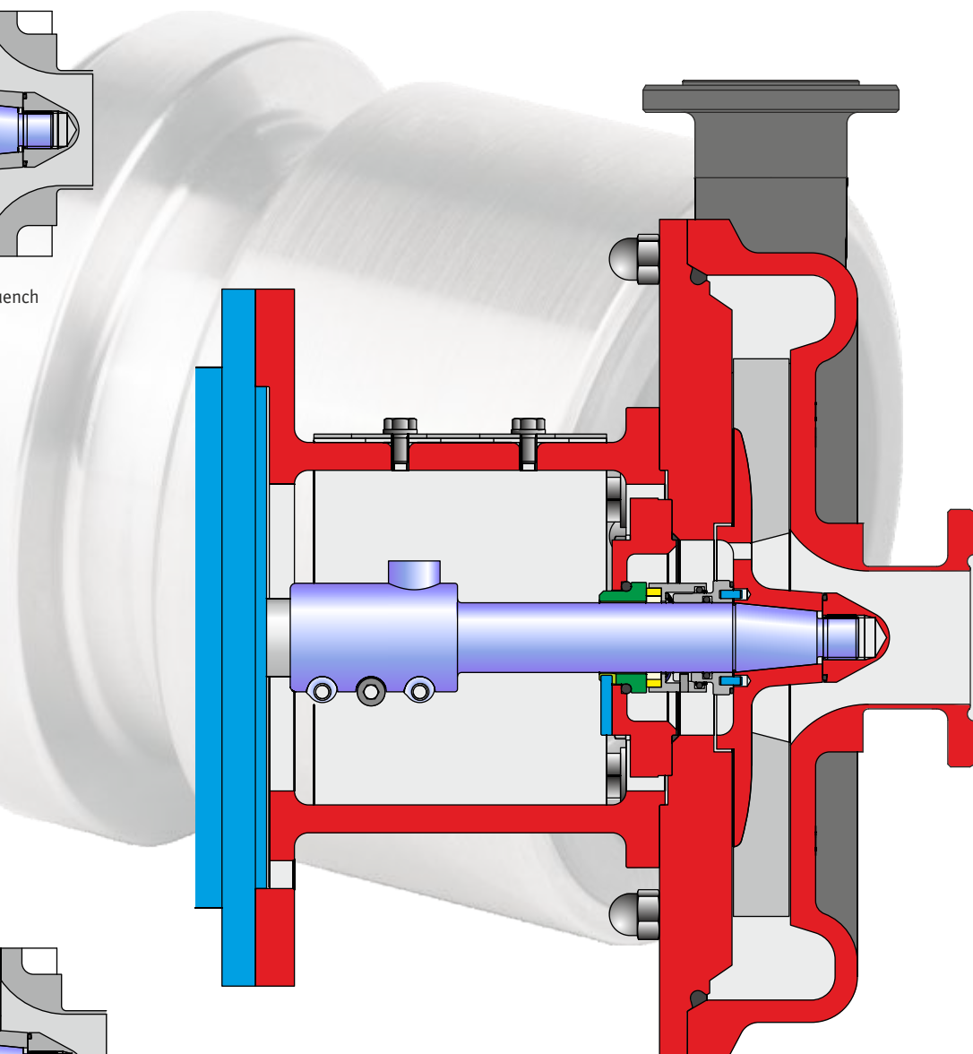
3. Buitenliggend mechanical seal
